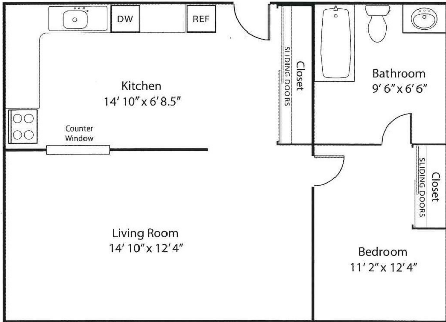
One Bedroom
